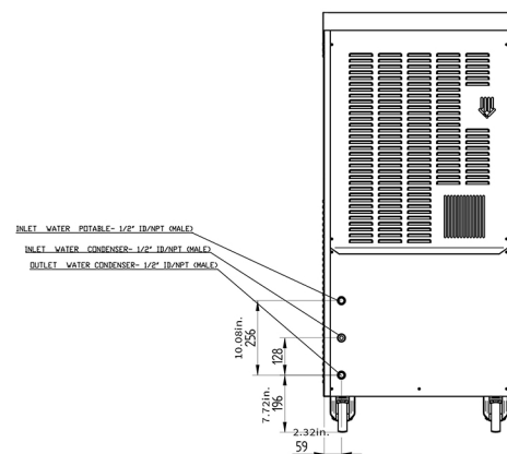
Rear Detail
