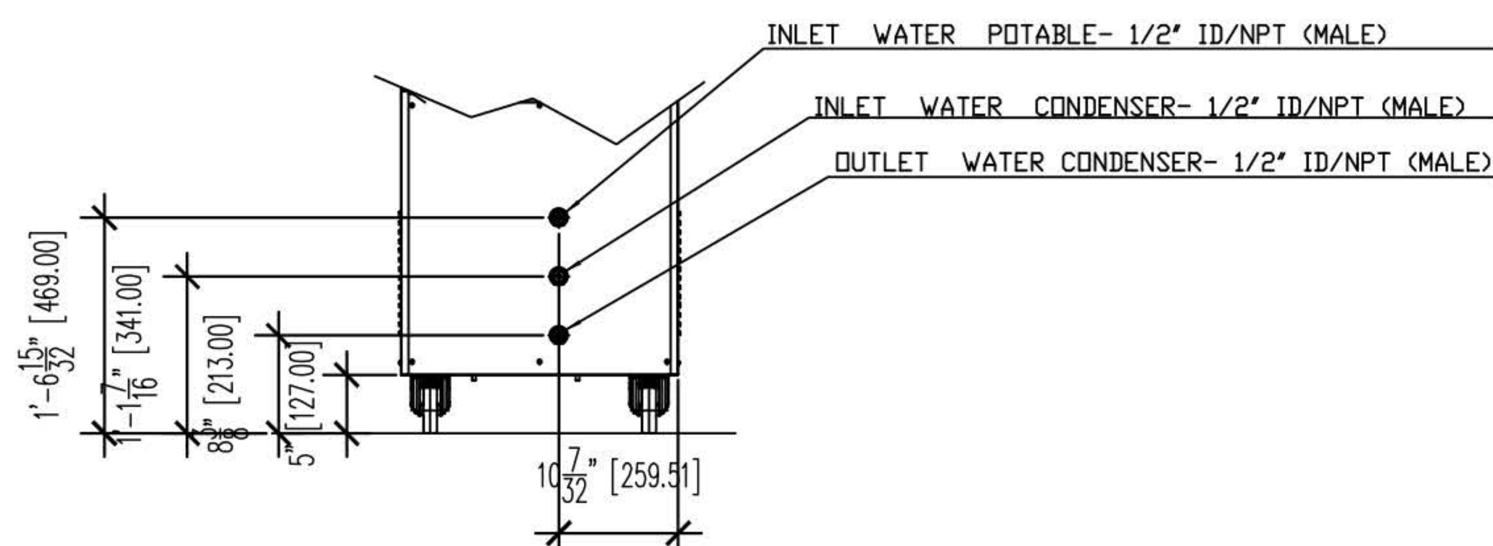
Rear Detail
