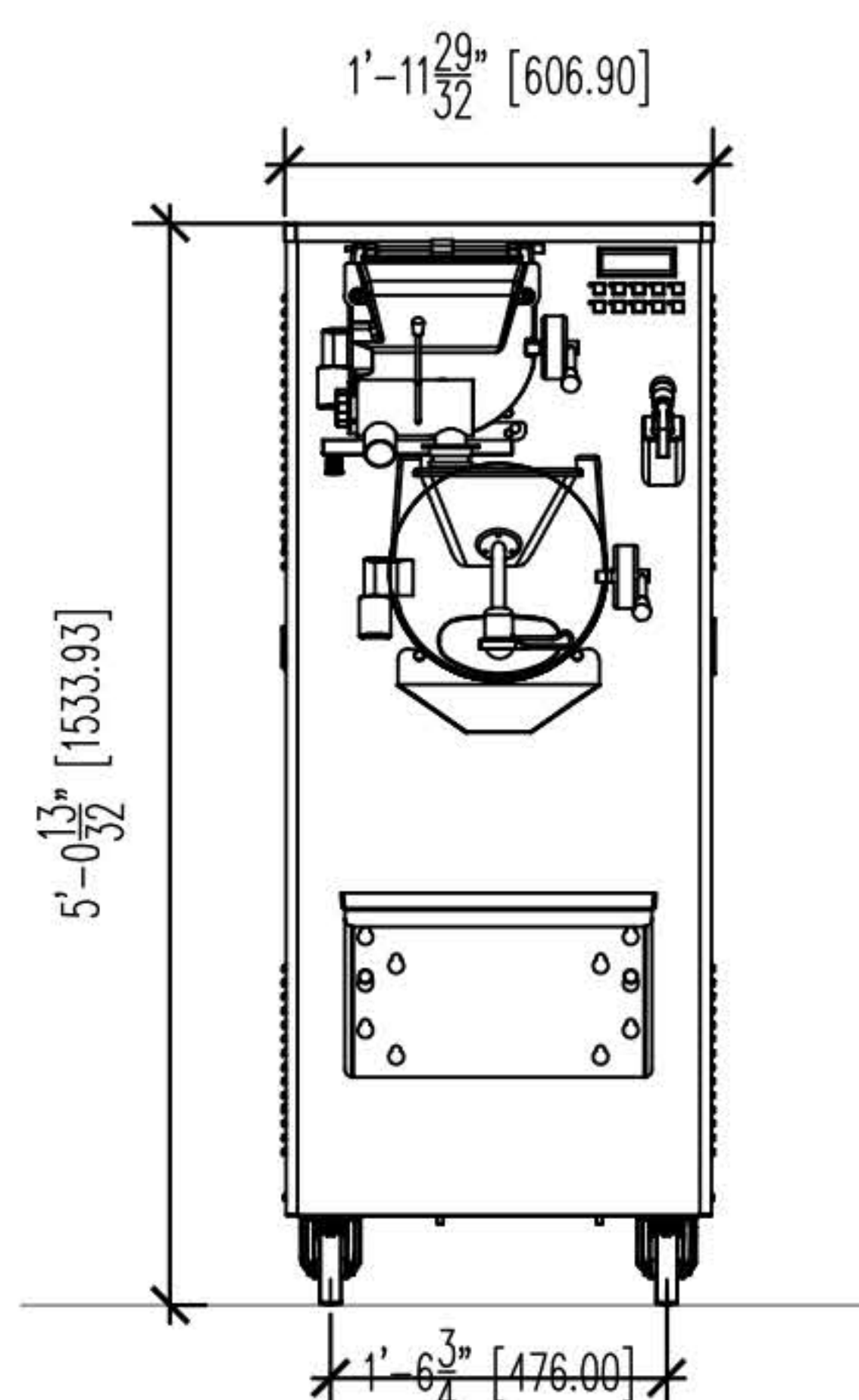
Front Elevation
