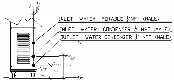
Rear Detail
