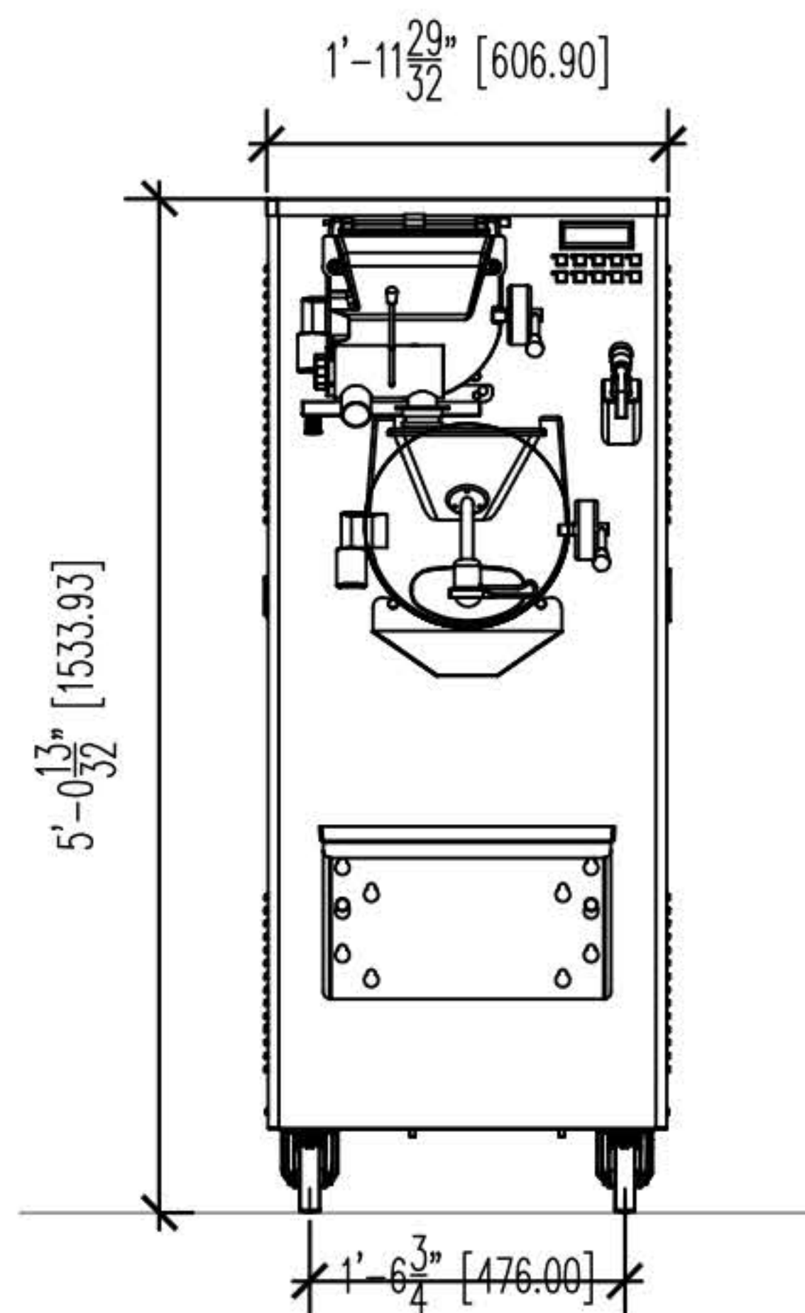
Front Elevation
