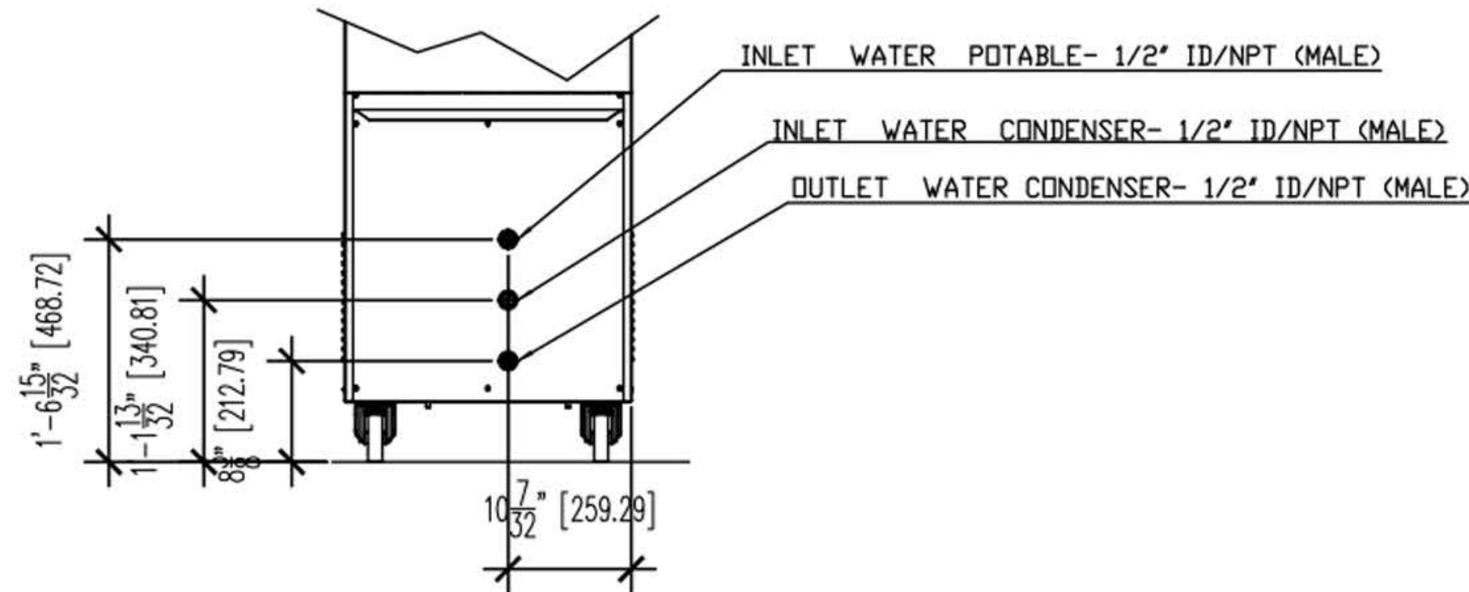
Side View
