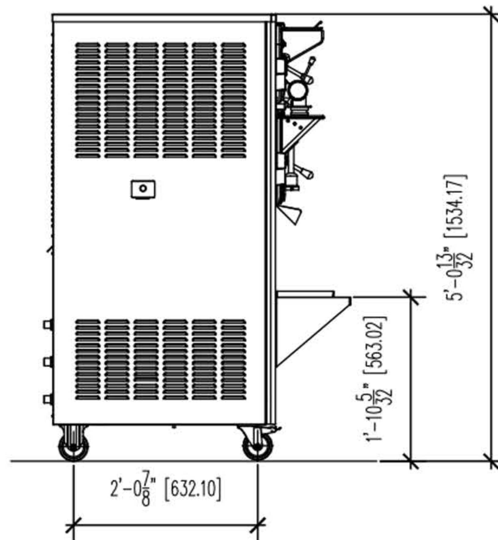
Side View
