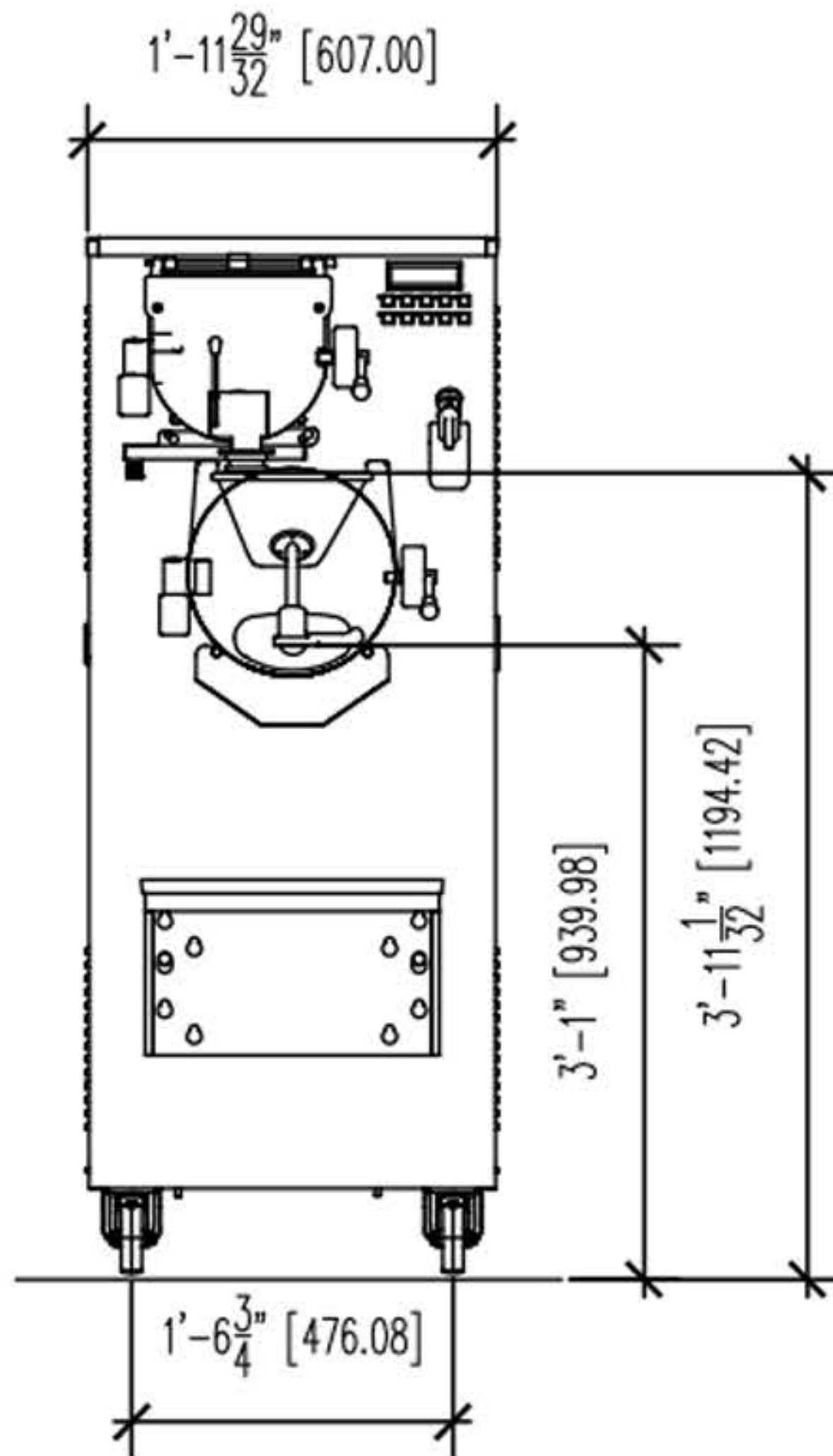
Front Elevation
