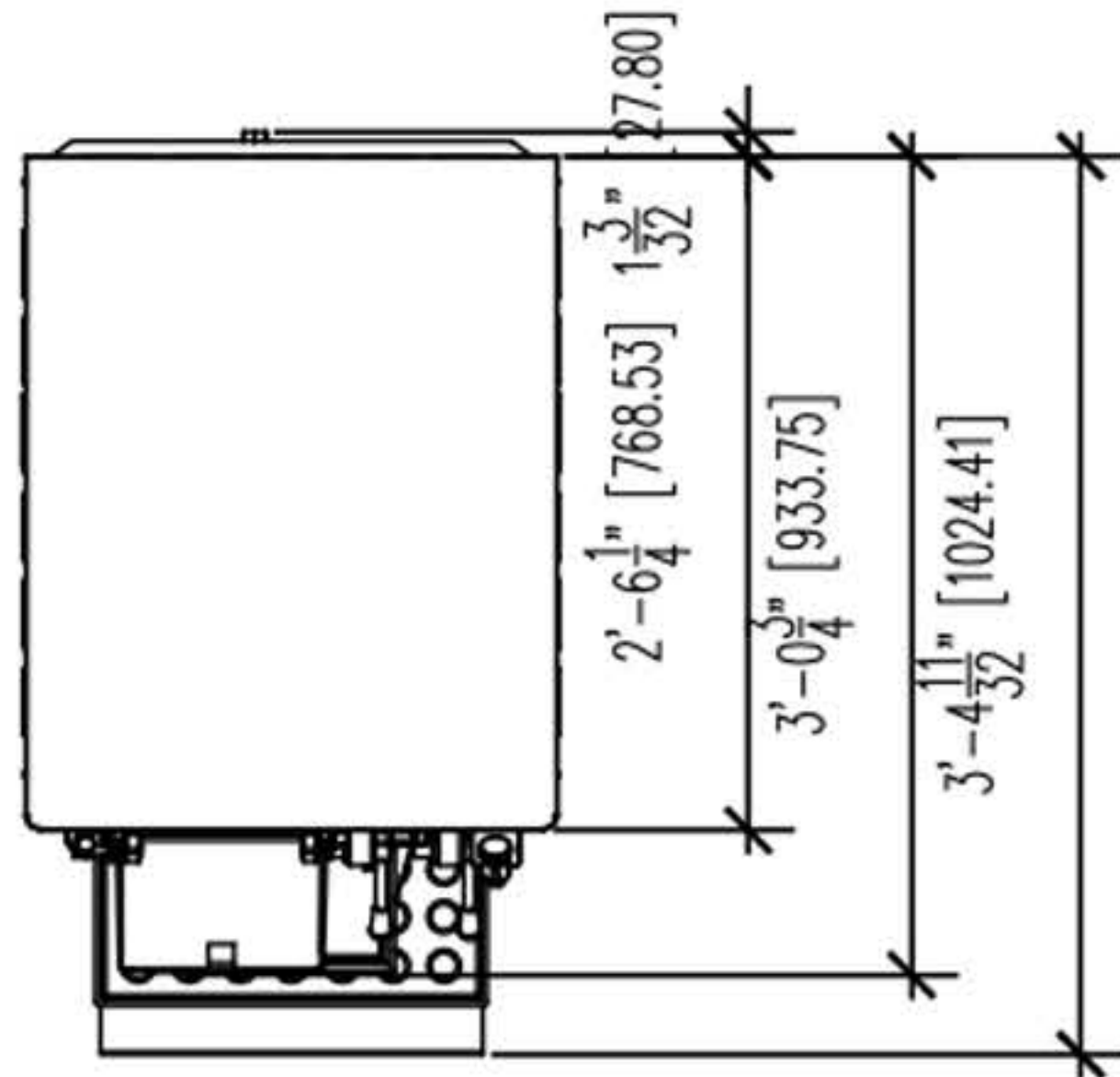
Front Elevation
